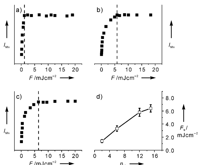
Figure 3. I_{Mn} as a function of laser fluence for the CdS/ZnS nanocrystals doped with a) 2 Mn ions, b) 12 Mn ions, and c) 15 Mn ions. d) F_s as a function of the average number of Mn ions n_{Mn} inside a dot.
